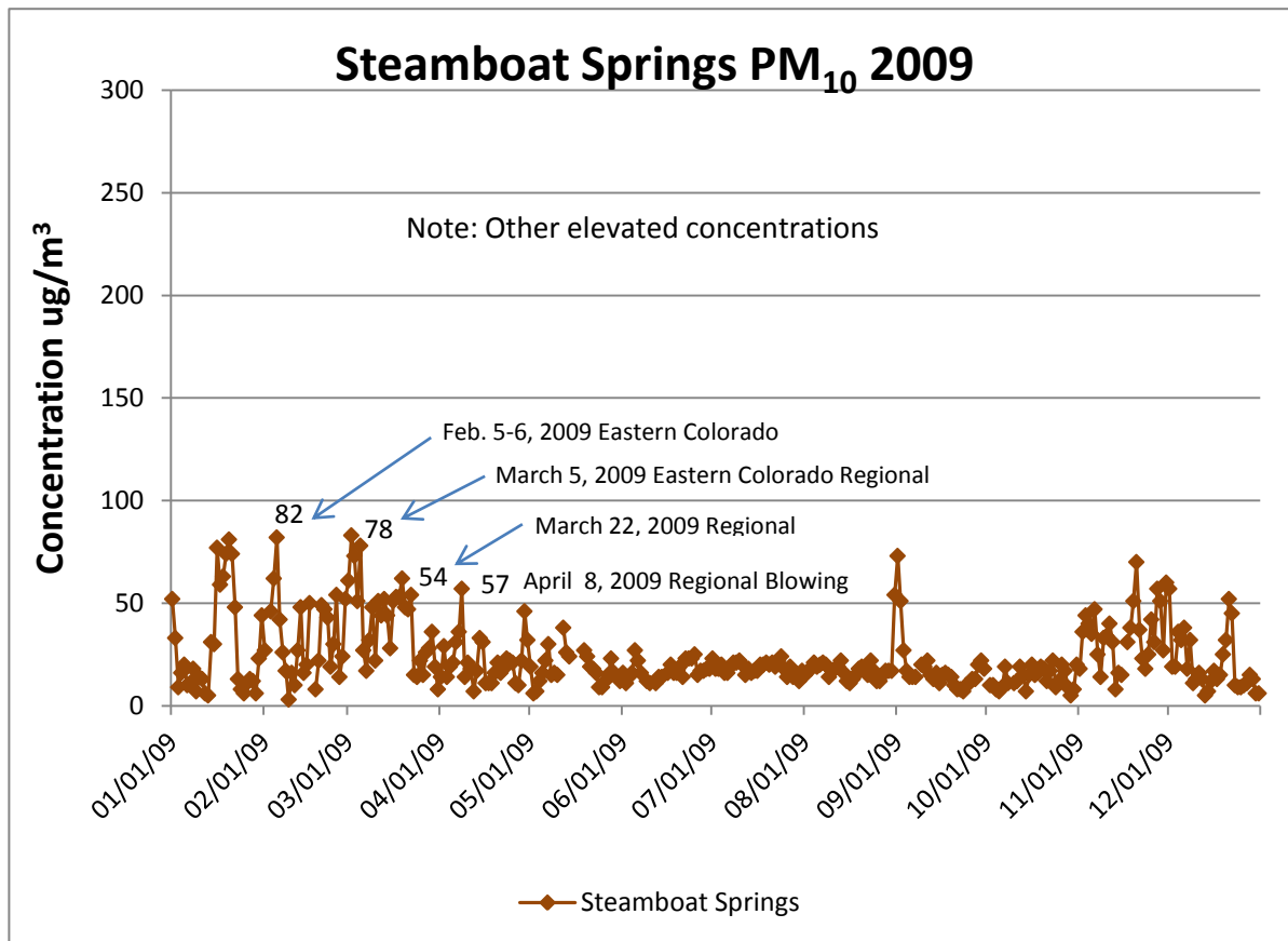
Figure 41. PM 10 Annual Concentrations in Steamboat Springs during 2009.
