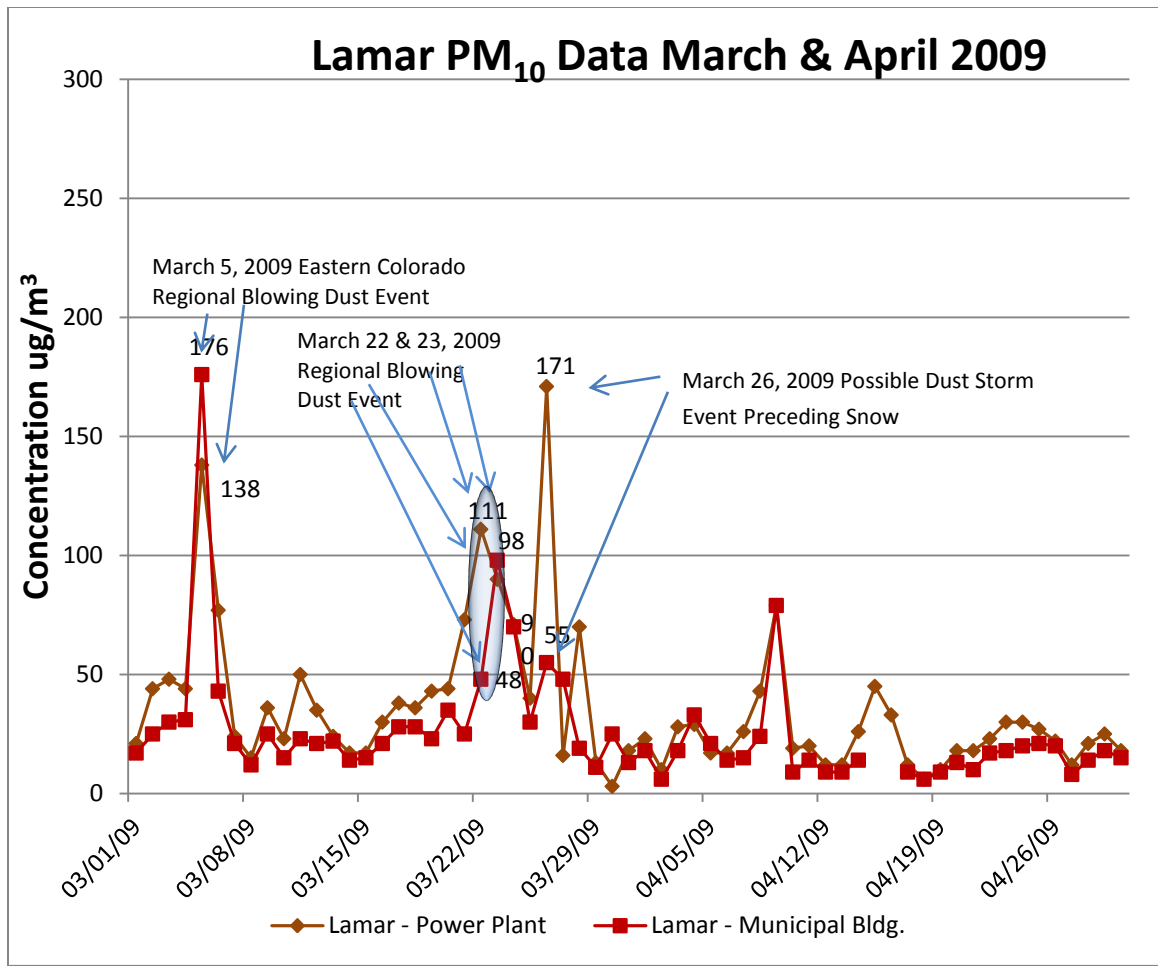
Figure 37. PM 10 Seasonal Concentrations in Lamar, March and April, 2009.
