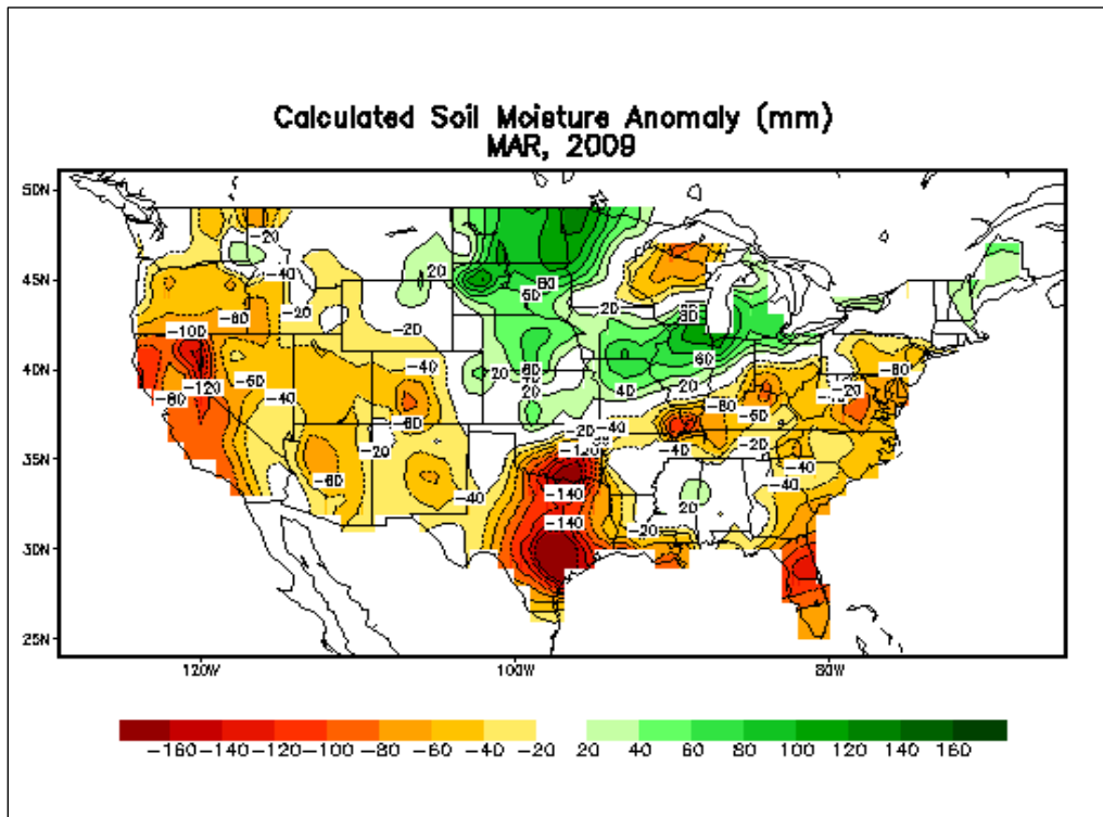
Figure 14. Calculated Soil Moisture Anomaly for March 2009 ( http://www.cpc.ncep.noaa.gov/cgi-bin/US_Soil-Moisture-Monthly.sh ).
