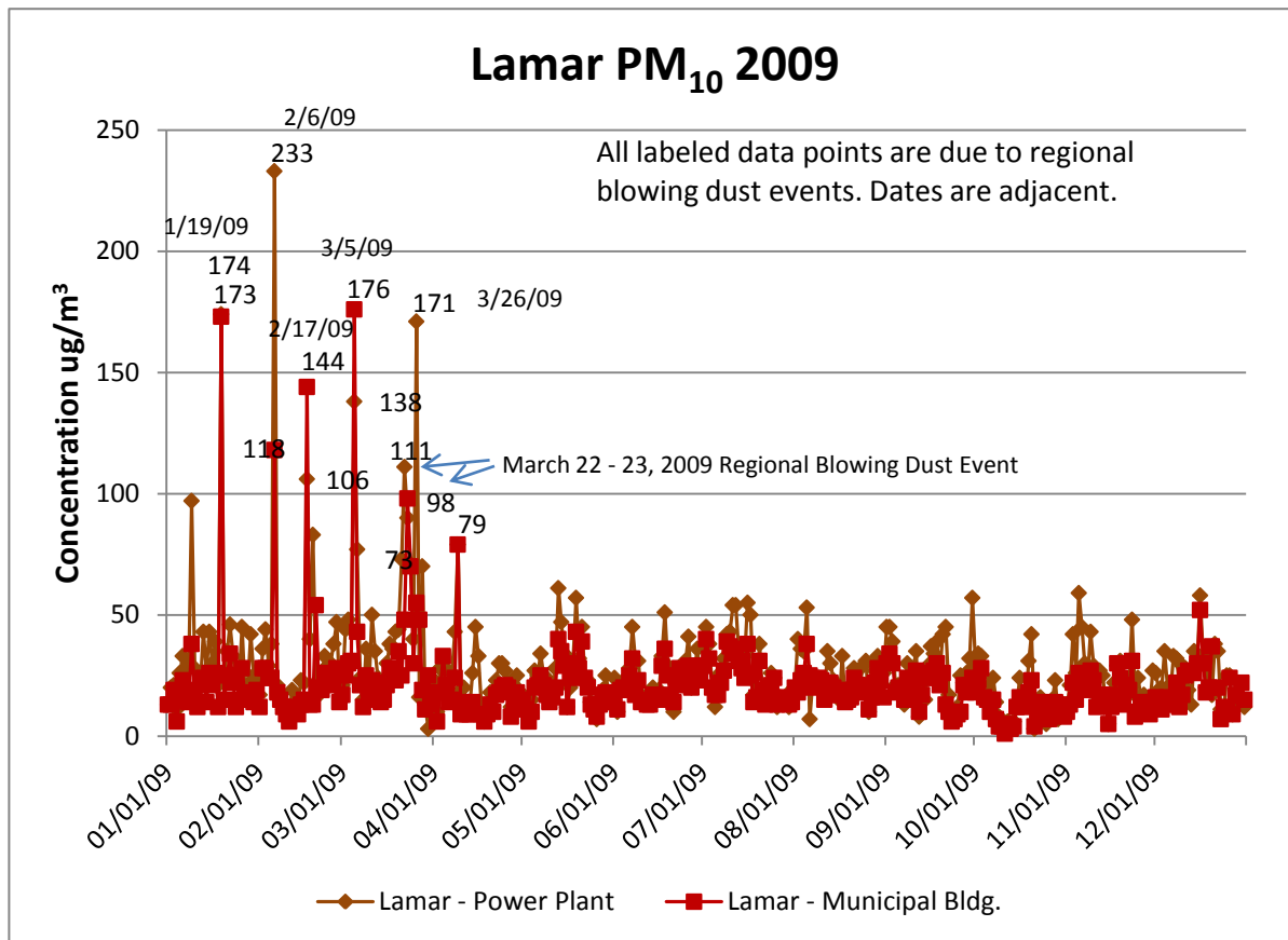
Figure 40. PM 10 Annual Concentrations in Lamar during 2009.
