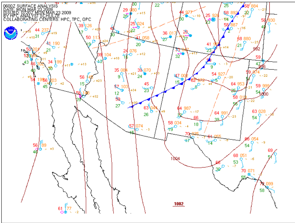
Southwest Surface analysis for 0600Z March 23, 2009, or 11PM MST March 22, 2009 http://nomads.ncdc.noaa.gov/nccep/NCEP .
