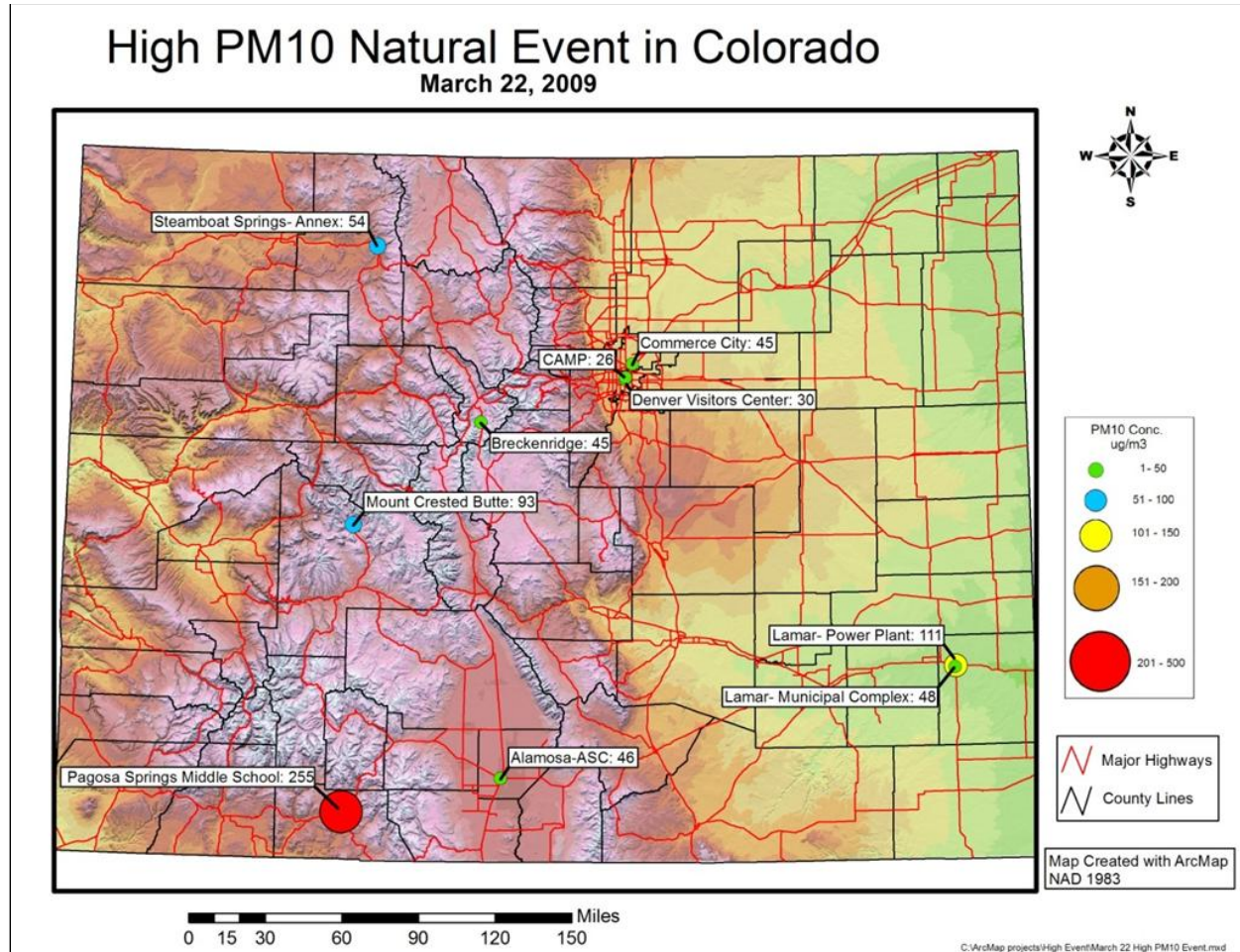
Figure 1. 24-hour PM 10 concentrations in µg/m 3 for March 22, 2009.
