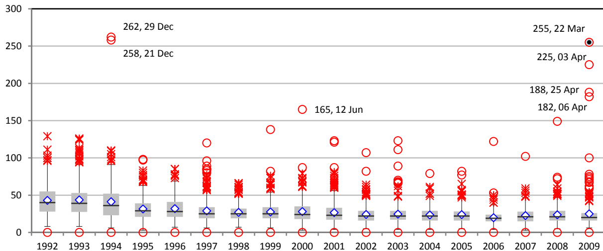
Figure 44. Annual Pagosa Springs \text{PM}_{10} Box and Whisker Plot.
