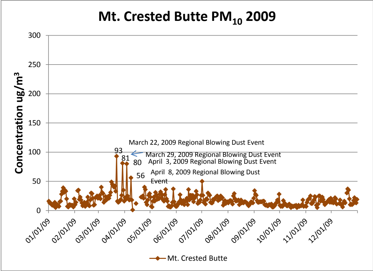
Figure 39. PM 10 Annual Concentrations in Mount Crested Butte during 2009.
