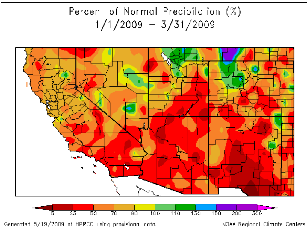
Figure 13. Percent of Normal Precipitation 1/1/2009 – 3/31/2009, source High Plains Regional Climate Center ( http://www.hprcc.unl.edu/maps/current/index.php?action=update_product&product=TDept ).
