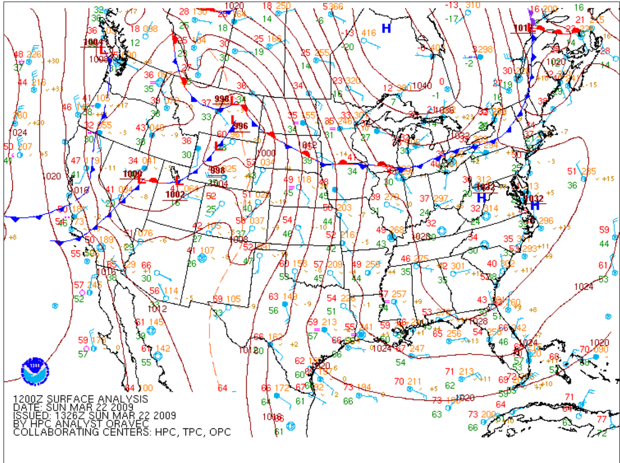
Figure 2. Surface analysis for 12Z March 22, 2009, or 5 AM MST March 22, 2009 (from National Weather Service fax maps http://nomads.ncdc.noaa.gov/ncep/ ).
