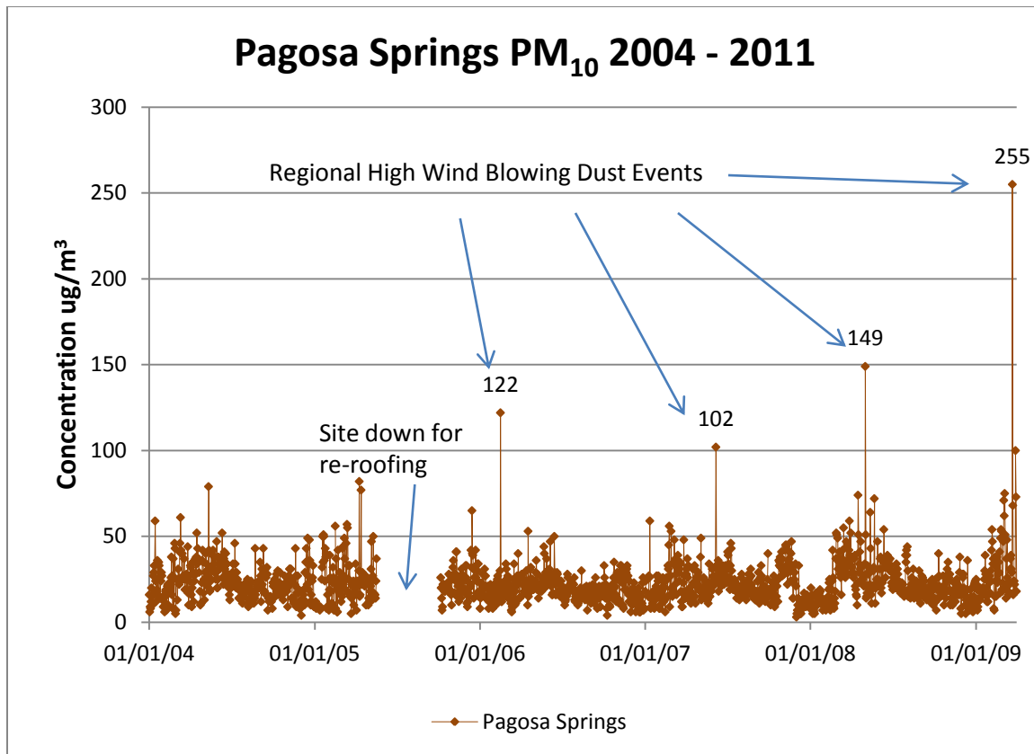
Figure 35. Five Year Time-Series Graph of PM 10 in Pagosa Springs
