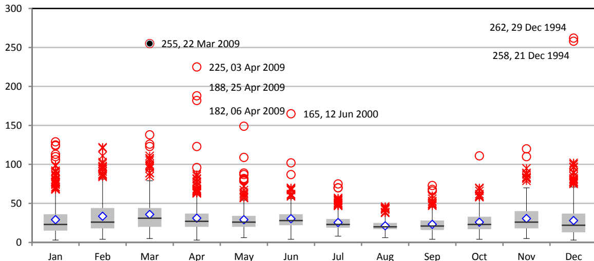
Figure 43. Monthly Pagosa Springs PM 10 Box and Whisker Plot.
