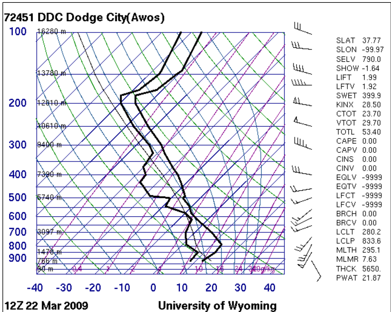
Figure 23. Dodge City sounding analysis for 12Z March 22, 2009, or 5 AM MST March 22, 2009 ( http://weather.uwyo.edu/upperair/sounding.html ).
