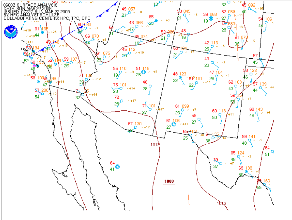
Southwest Surface analysis for 0600Z March 22, 2009, or 11 PM MST March 21, 2009 ( http://nomads.ncdc.noaa.gov/nccep/NCEP ).
