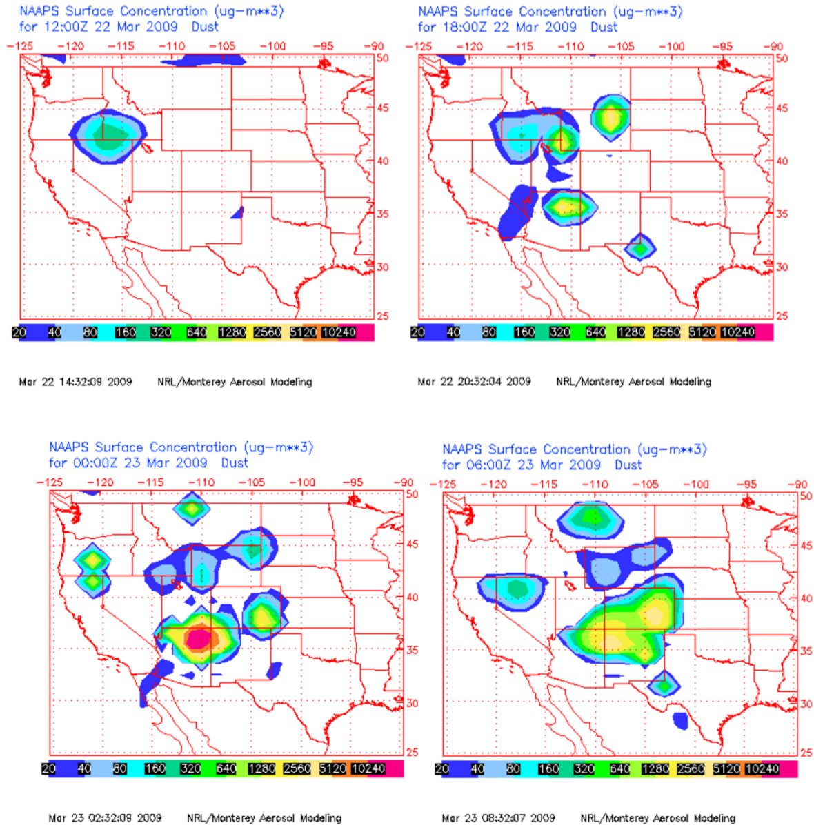
Figure 32. NAAPS forecasted dust concentrations for March 22, 2009 (source: http://www.nrlmry.navy.mil/flambe-bin/aerosol/display_directory_aer2?DIR=/web/aerosol/public_html/global/ops_01/wus/ ).
