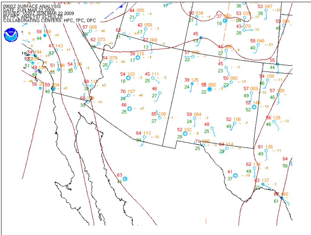
Southwest Surface analysis for 0900Z March 22, 2009, or 2 AM MST March 22, 2009 ( http://nomads.ncdc.noaa.gov/nccep/NCEP ).
