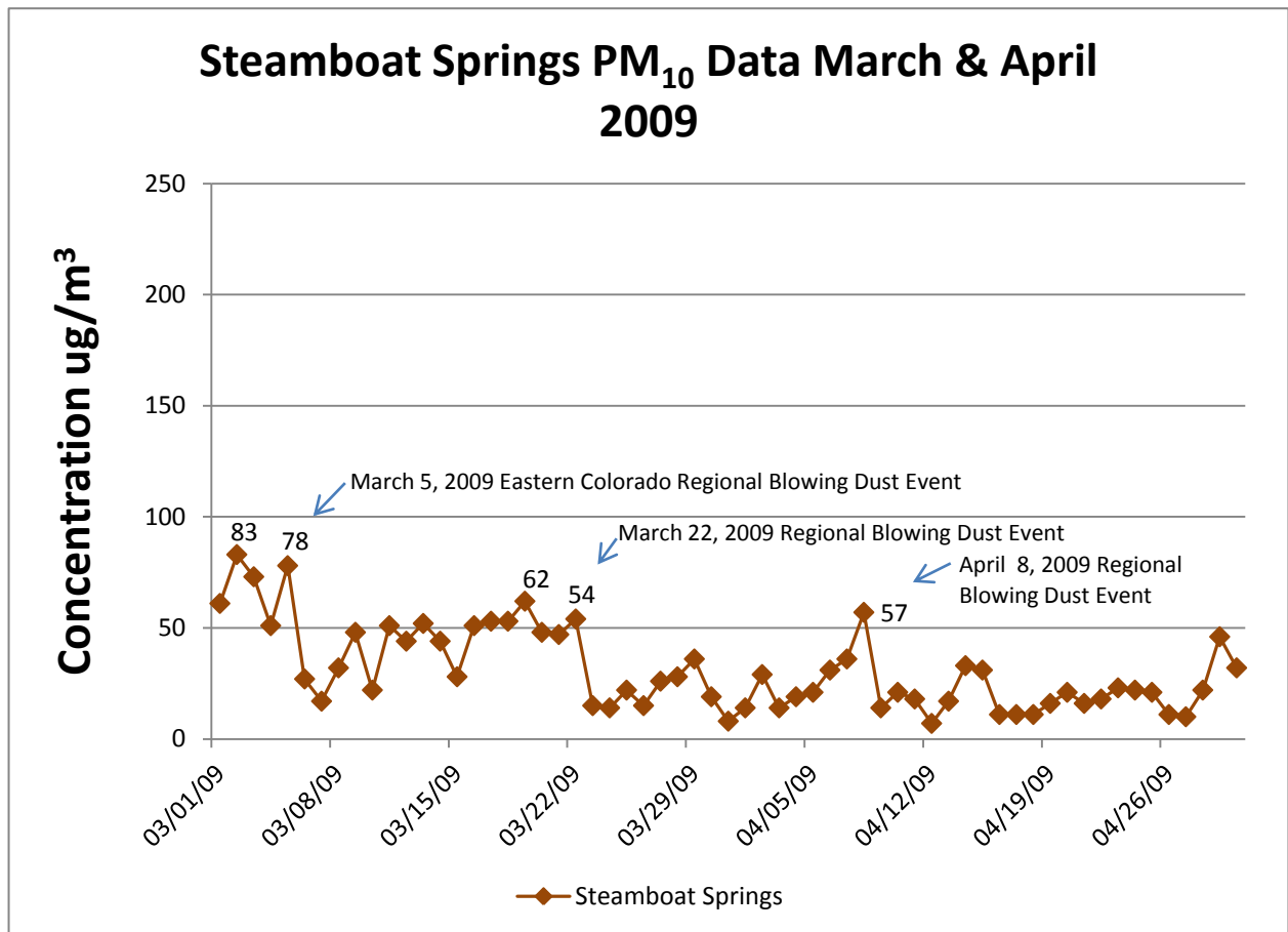
Figure 38. PM 10 Seasonal Concentrations in Steamboat Springs, March and April, 2009.
