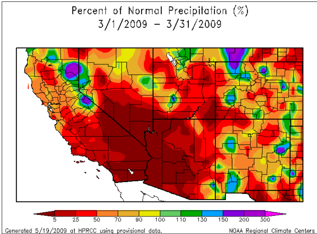
Figure 12. Percent of Normal Precipitation 3/1/2009 – 3/31/2009, source High Plains Regional Climate Center ( http://www.hprcc.unl.edu/maps/current/index.php?action=update_product&product=TDept ).
