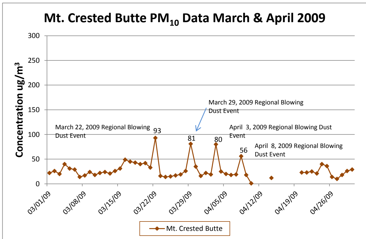
Figure 36. PM 10 Seasonal Concentrations in Mount Crested Butte, March and April, 2009.
