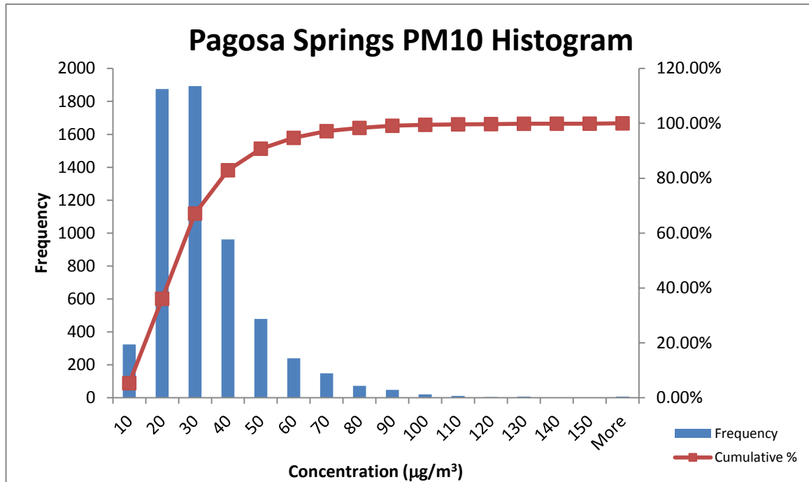
Figure 42. Pagosa Springs PM 10 Histogram.
