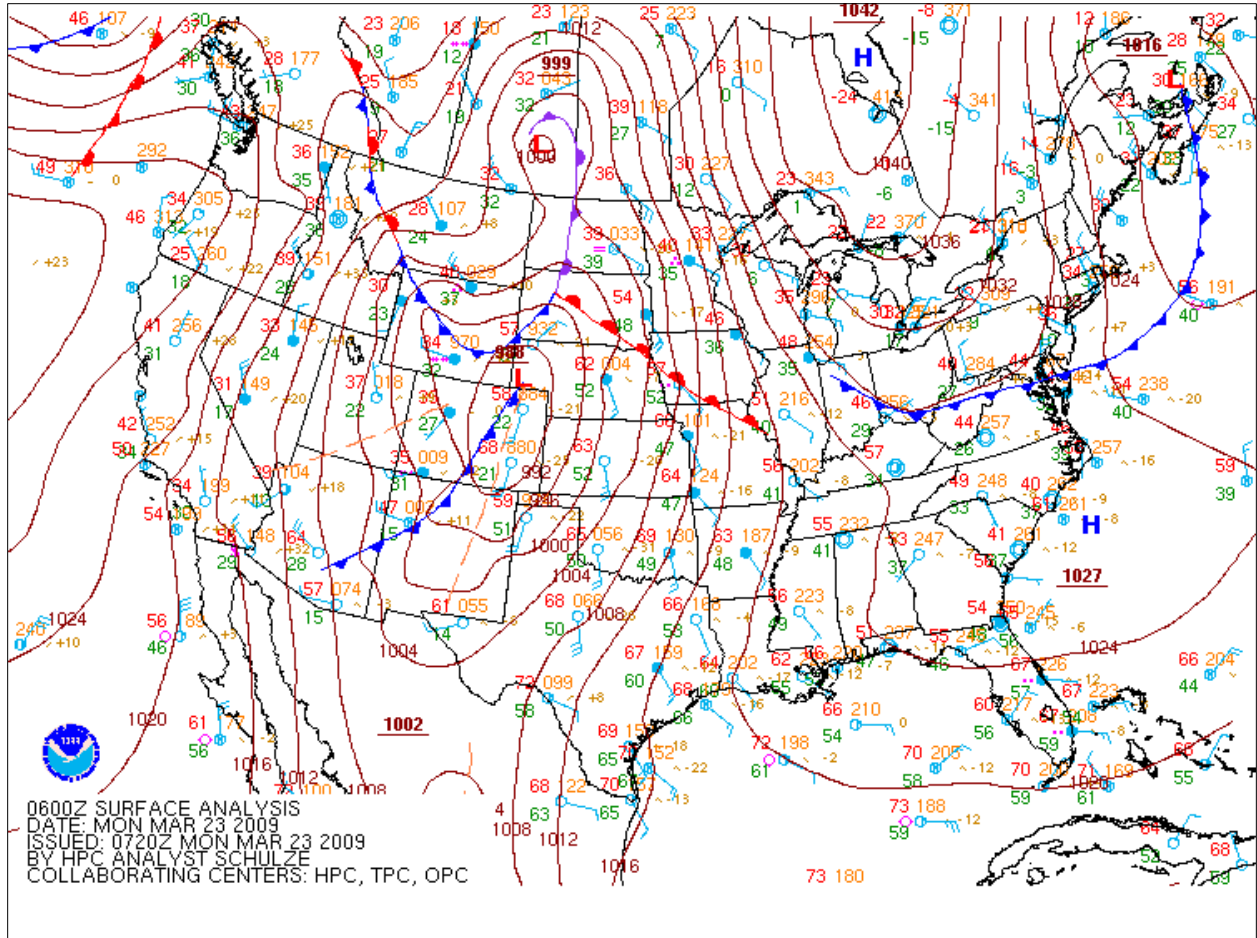
Figure 3. Surface analysis for 06Z March 23, 2009, or 11 PM MST March 22, 2009 (from National Weather Service fax maps http://nomads.ncdc.noaa.gov/ncep/NCEP ).
